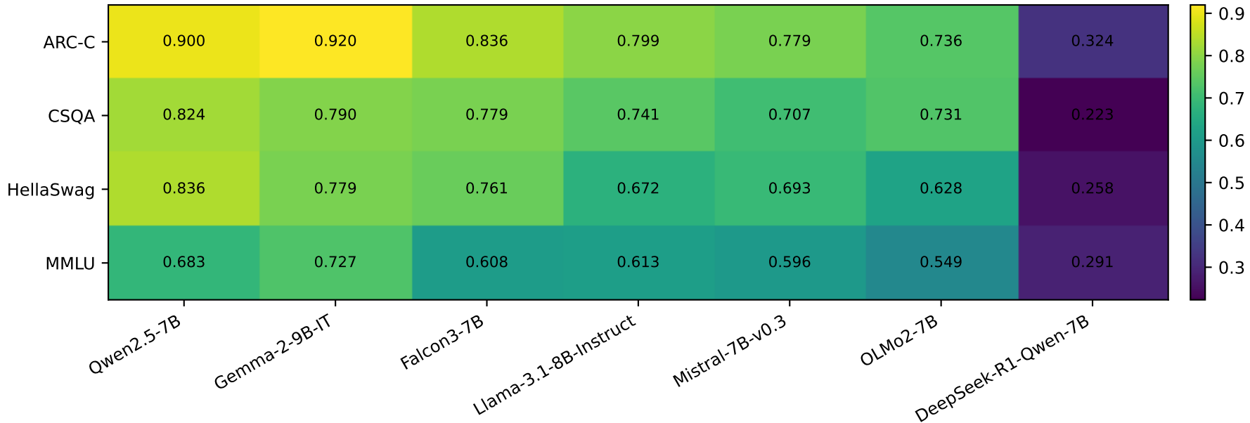
Base MCQ accuracy across final scaling audit
