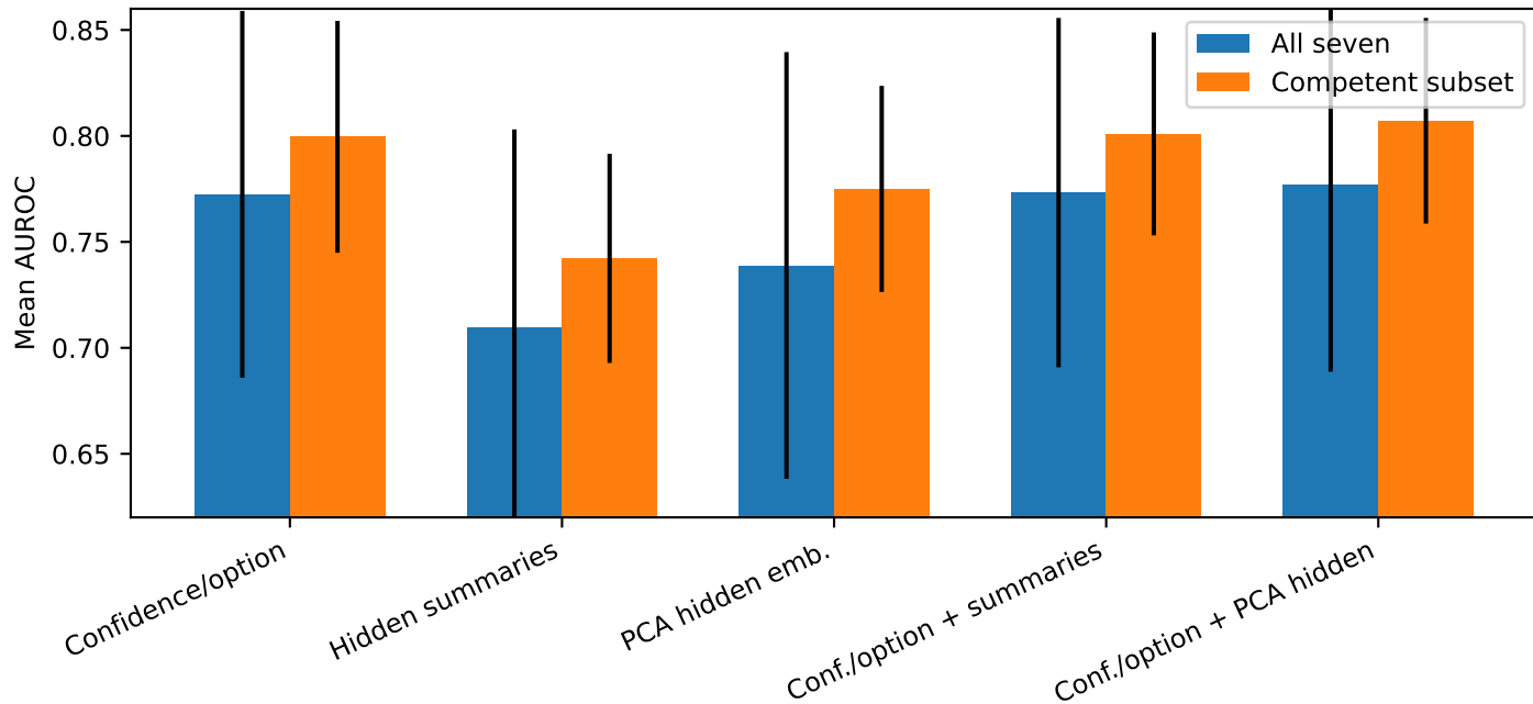
Reliability prediction by feature family
