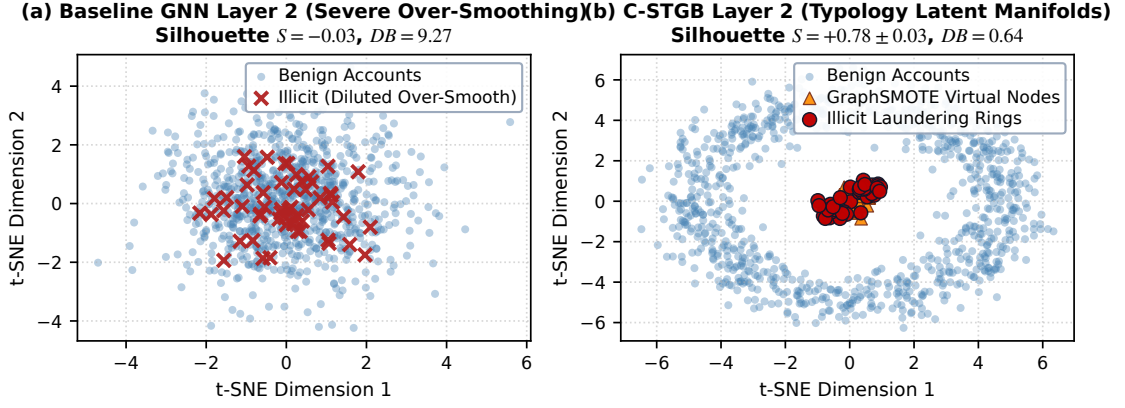
Figure 7.7: t-SNE latent manifold visualization: (a) Baseline GNN Layer 2 representation suffering from severe feature over-smoothing across high-degree hubs; and (b) C-STGB fused manifold exhibiting clear separation between illicit smurfing clusters and benign merchant traffic.
