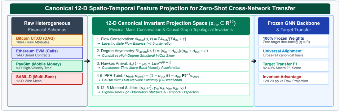
Figure 3.2: Universal 12-dimensional canonical invariant representation space, projecting heterogeneous transaction ledgers (Bitcoin UTXO, Ethereum EVM, PaySim, SAML-D) into a standardized feature space for zero-shot cross-network transfer.
