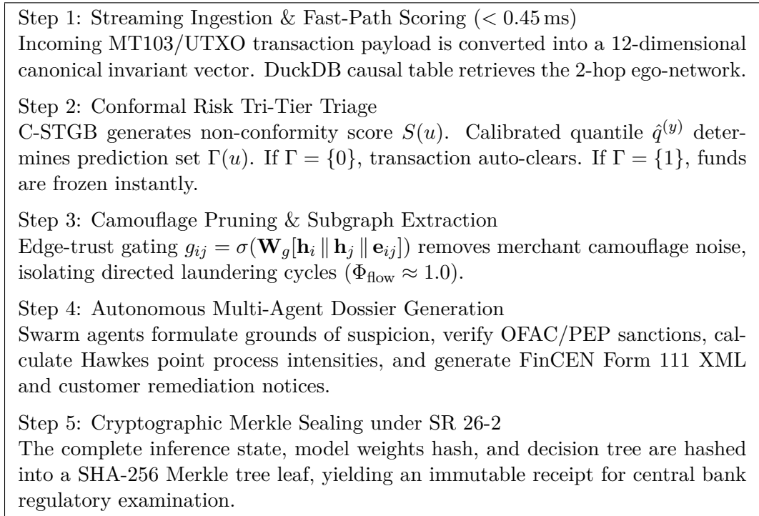
Figure D.1: End-to-end operator investigation lifecycle enforced by the Intelligent-AML platform.
