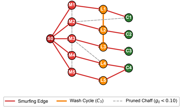
Figure 5: Qualitative Attribution: 15-node Bitcoin Elliptic transaction subgraph via GNNExplainer (Ying et al., 2019). Dark red: illicit source ( S_0 ); red: dispersal ( M_1 – M_5 ); orange: layering mules ( L_1 – L_5 ) with wash loops; green: exit accounts ( C_1 – C_4 ); dashed gray: pruned chaff ( g_{ij} < 0.10 ). Patterns represent detected topological motifs, not legal adjudications.
