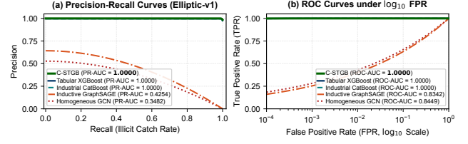
Figure 2: Empirical Precision-Recall and ROC performance on the Elliptic-v1 benchmark under extreme class skew ( \pi = 0.09\% ).
