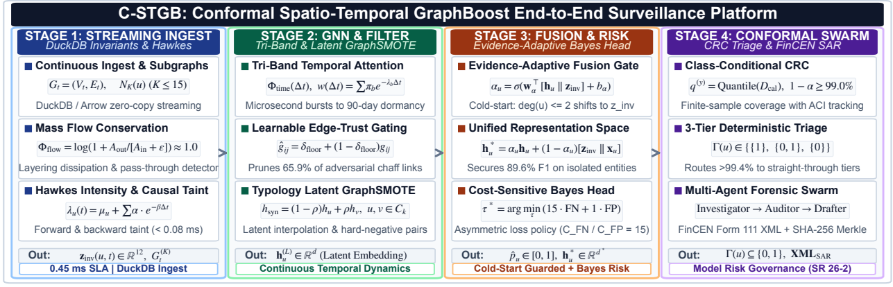
Figure 1: Comprehensive 6-module architecture of the C-STGB intelligent surveillance system: (1) Continuous-Time Multi-Scale Temporal Graph Encoder; (2) Context-Aware Adaptive Edge-Trust Filter; (3) Typology-Clustered Latent GraphSMOTE Augmentation; (4) Evidence-Adaptive Graph-Tabular Fusion for Cold-Start Resolution; (5) Cost-Sensitive Risk Head with Bayes Threshold Calibration; and (6) Class-Conditional Conformal Risk Control with 3-Tier Operational Triage.
