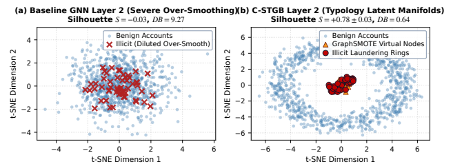
Figure 3: Latent manifold t-SNE projection: baseline GNN (left) exhibits severe feature over-smoothing around commercial hubs, whereas C-STGB under Typology GraphSMOTE (right) induces dense, distinct clustering of confirmed illicit topologies ( K = 4 ) with sharp boundary separation.
