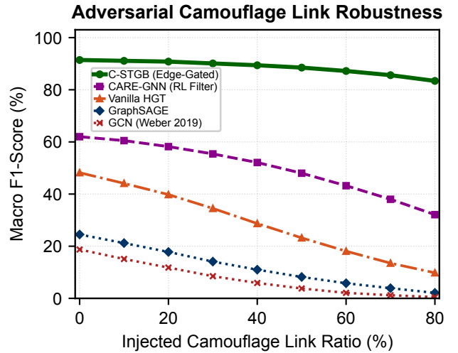
Figure 4: Adversarial Camouflage Robustness: Macro F1 retention across perturbation ratios \rho \in [0, 0.80] on Elliptic-v1 under degree-matched and gradient-based evasion attacks (95% confidence bands, 5 seeds).
