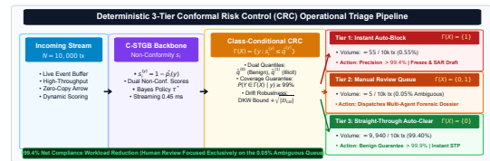
Figure S1: Operational 3-Tier Queue Mapping and Conformal Risk Control triage workflow under within-class exchangeability. Ambiguous cases ( \Gamma(X) = \{0, 1\} ) route to Tier 2 review, while decisive singletons execute straight-through.
