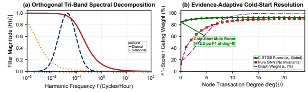
Figure S6: Evidence-adaptive gating dynamics \alpha_u and spectral cold-start representation analysis across network density regimes.
