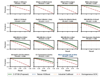
Comprehensive Small-Multiples Precision-Recall Curves across ALL 14 Empirical Datasets
