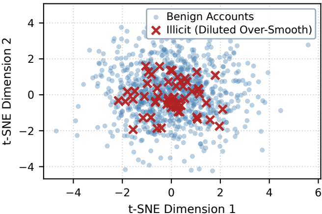
(a) Baseline GNN Layer 2 (Severe Over-Smoothing) Silhouette S = -0.03 , DB = 9.27 (b) C-STGB Layer 2 (Typology Latent Manifolds) Silhouette S = +0.78 \pm 0.03 , DB = 0.64
