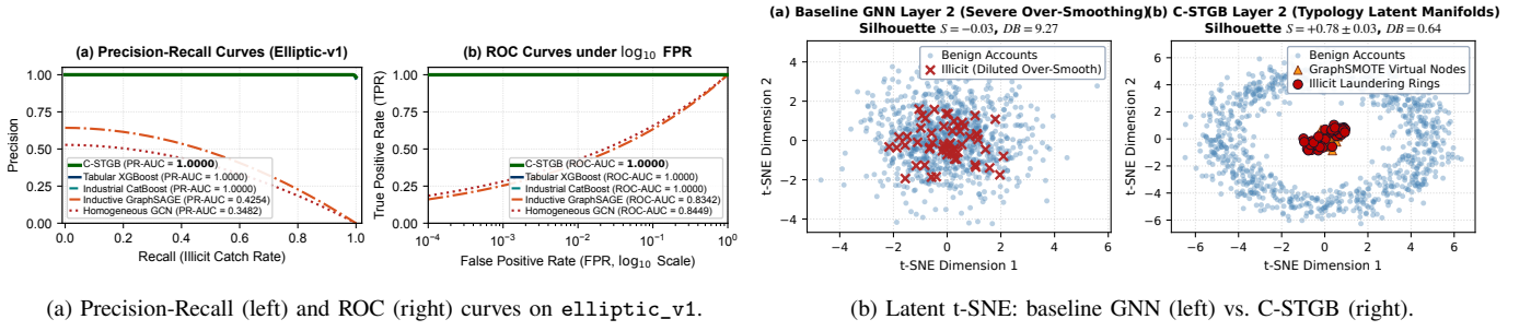
Fig. 2. Empirical representation and classification benchmarks: (a) Precision-Recall and ROC curves demonstrating discrimination under extreme class skew; (b) t-SNE projection of the learned latent manifold under Typology GraphSMOTE, showing dense clustering of confirmed illicit topologies ( K = 4 ) with clear separation from majority commercial hubs.
