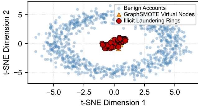
(b) STGB Layer 2 (Typology Latent Manifolds)
