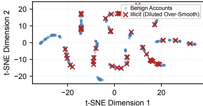
(a) Baseline GNN Layer 2 (Severe Over-Smoothing) Silhouette S = -0.03 , DB = 9.23
