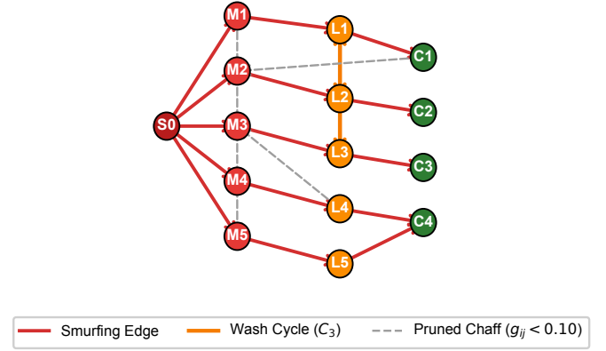
Fig. 4. Qualitative Attribution: 15-node Bitcoin Elliptic subgraph via GNNExplainer [38]. Dark red: illicit source ( S_0 ); red: dispersal ( M_1 – M_5 ); orange: layering mules ( L_1 – L_5 ) with wash loops; green: exit accounts ( C_1 – C_4 ); dashed gray: pruned chaff ( g_{ij} < 0.10 ). Motifs, not legal adjudications.
