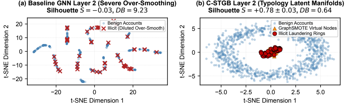
Figure 7.7: t-SNE latent manifold visualization: (a) Baseline GNN Layer 2 representation suffering from severe feature over-smoothing across high-degree hubs; and (b) C-STGB fused manifold exhibiting clear separation between illicit smurfing clusters and benign merchant traffic.
