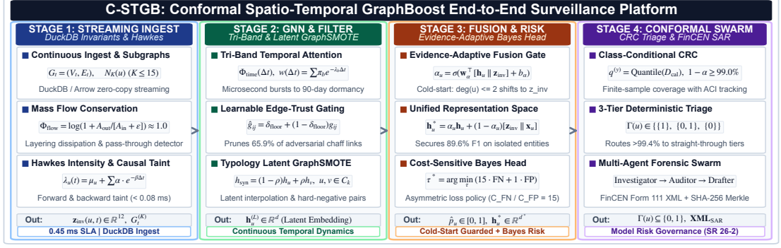
Figure 3.1: End-to-End Architectural Dataflow of C-STGB v2, detailing data ingestion, continuous-time temporal encoding, learnable edge-trust gating, latent manifold oversampling, evidence-adaptive fusion, and conformal risk control.
