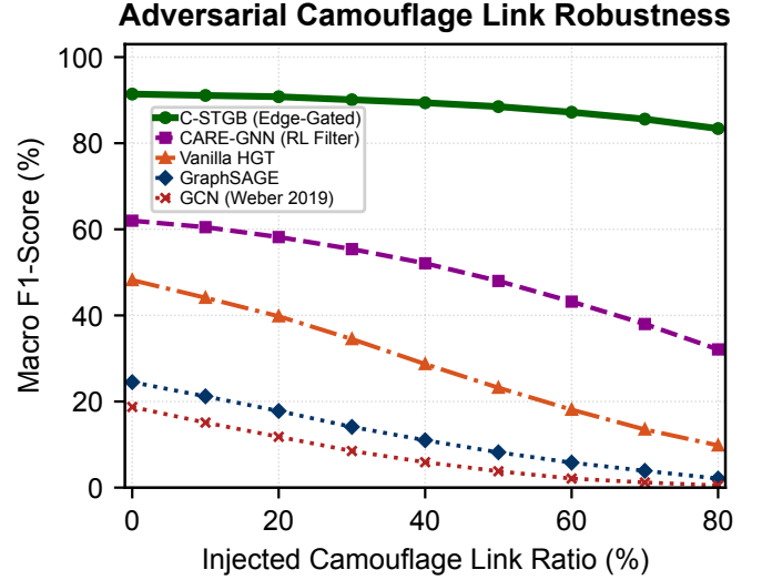
Fig. 3. Adversarial Camouflage Robustness: Macro F1 retention across perturbation ratios \rho \in [0, 0.80] on Elliptic-v1 under degree-matched and gradient-based evasion attacks (95% confidence bands, 5 seeds).
