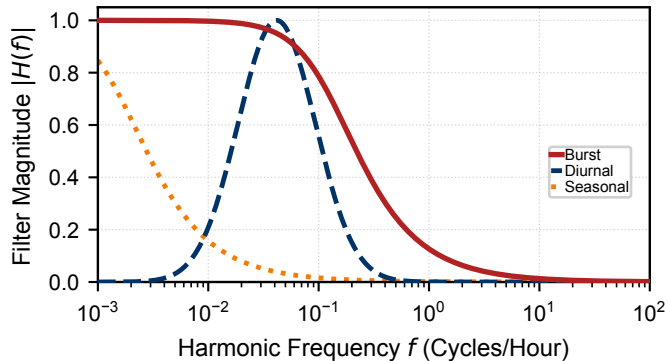
(a) Orthogonal Tri-Band Spectral Decomposition
