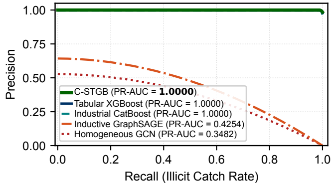
(a) Precision-Recall Curves (Elliptic-v1)
