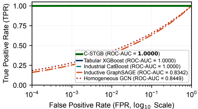
(b) ROC Curves under \log_{10} FPR
