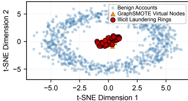
(b) STGB Layer 2 (Typology Latent Manifolds) Silhouette S = +0.78 \pm 0.03 , DB = 0.64
