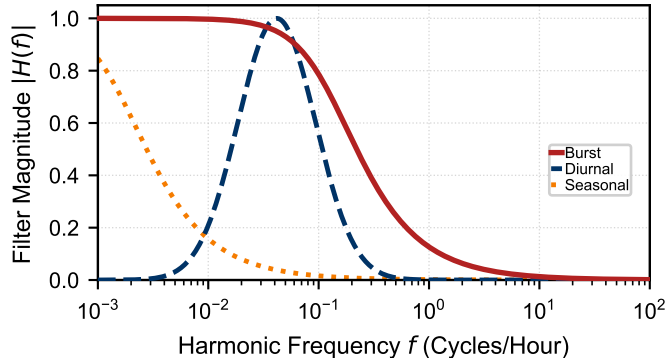
(a) Orthogonal Tri-Band Spectral Decomposition
