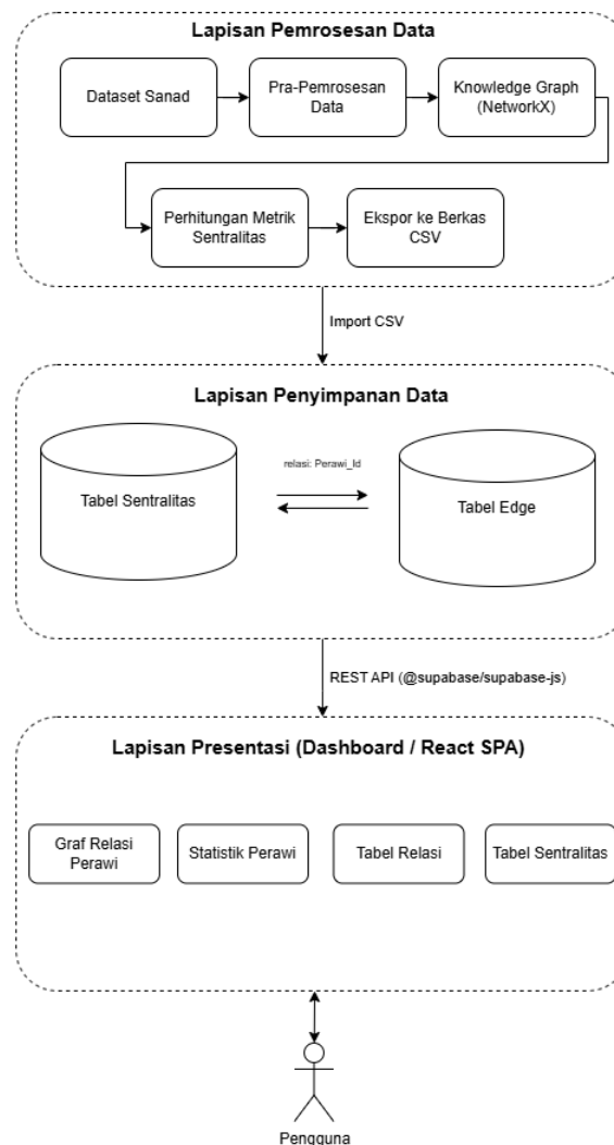
Gambar 3.3. Arsitektur sistem tiga lapis ( three-tier architecture )
