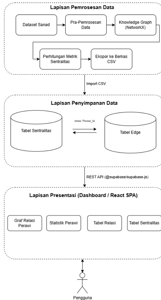
Gambar 3.2. Arsitektur sistem tiga lapis ( three-tier architecture )
