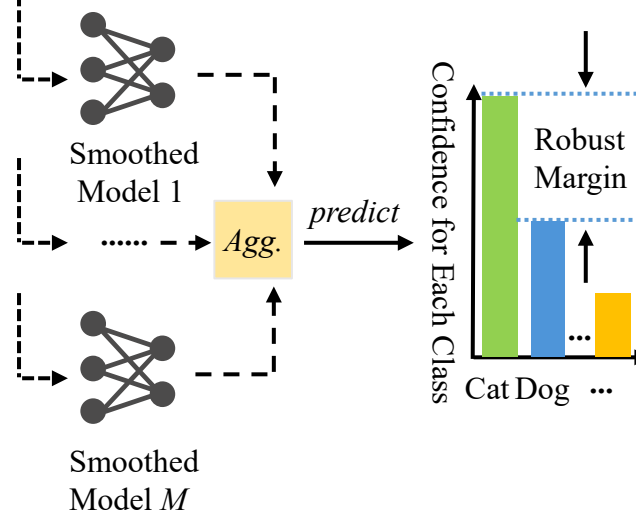
Stage 2: Cert-SSBD Inference
