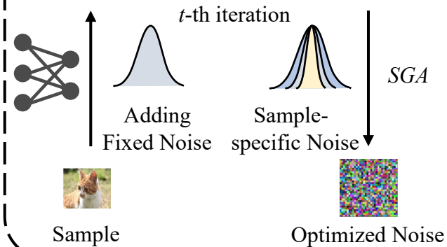
Stage 1: Cert-SSBD Training
