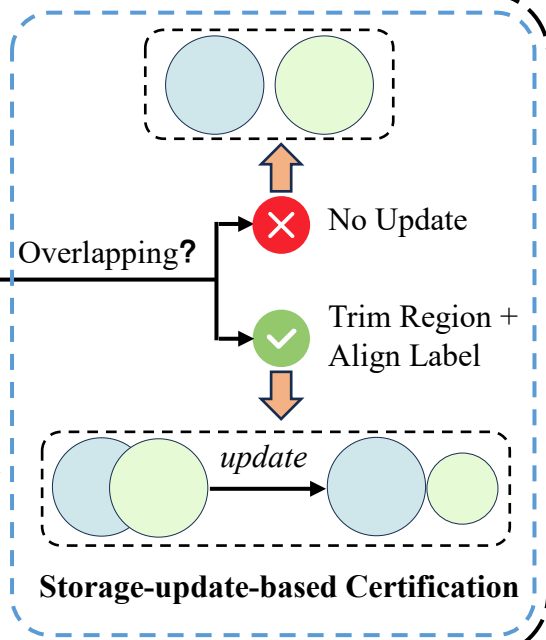
Stage 2: Cert-SSBD Inference
