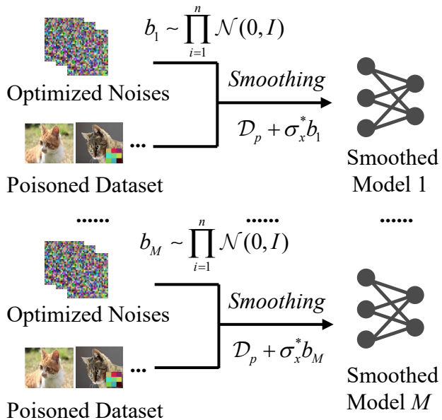
Stage 1: Cert-SSBD Training
