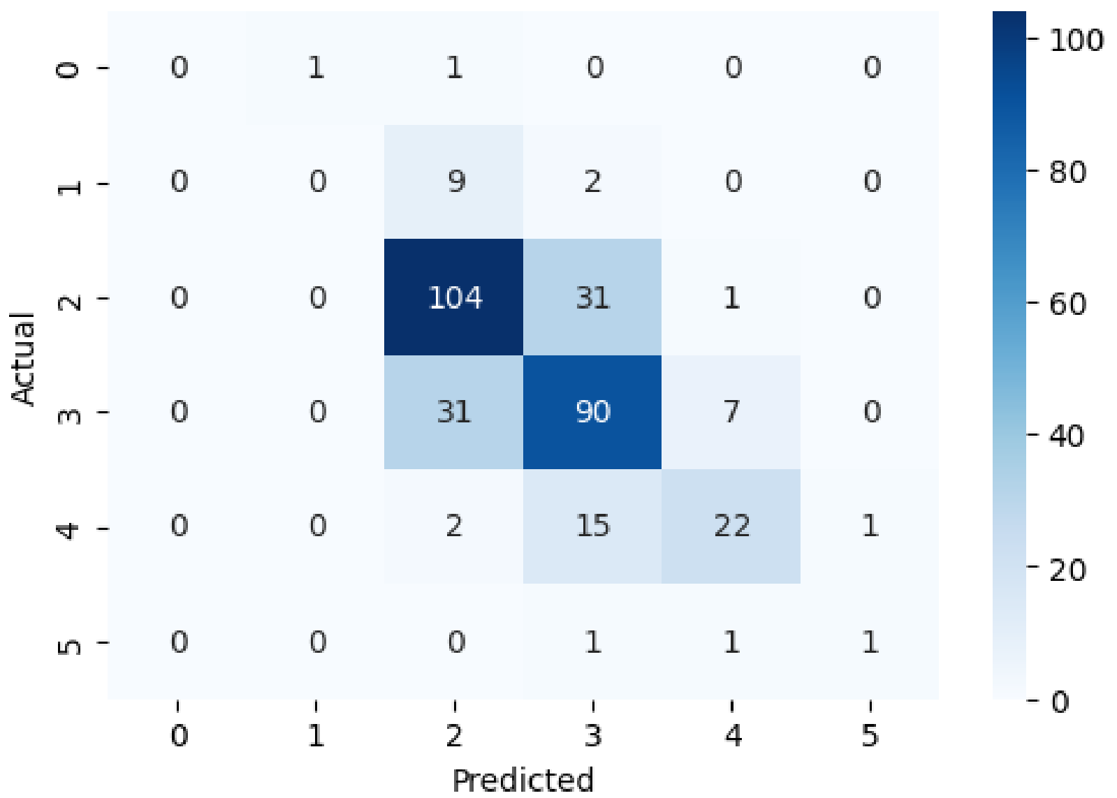
Confusion Matrix - Random Forest Classifier
