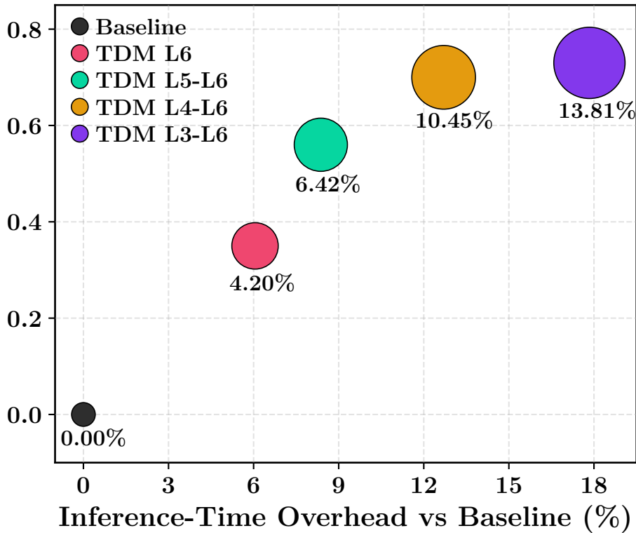
BLEU Gain vs Baseline
