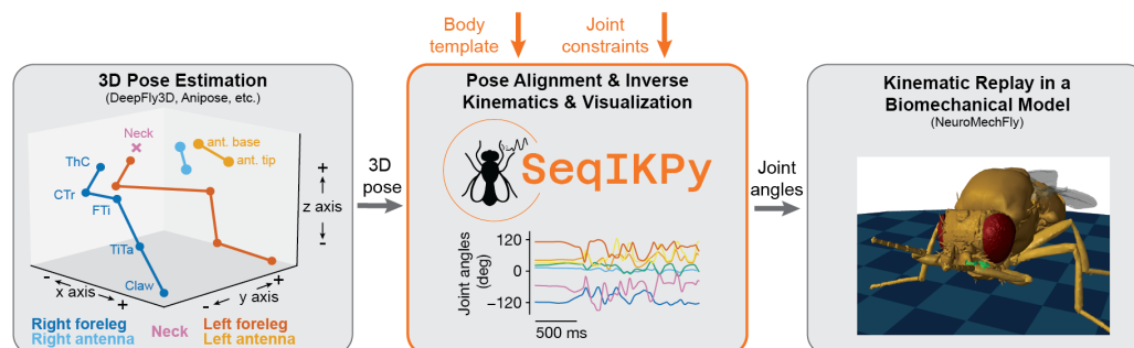
Figure 1: Overview of the SeqIKPy pipeline. (Left) Pose estimation tools (e.g., DeepFly3D and Anipose) estimates 3D positions of body key points. (Middle) SeqIKPy aligns these points to a body template, performs sequential inverse kinematics using joint constraints to calculate joint angles. (Right) The computed joint angles can be used to replay measured motions in biomechanical models, such as NeuroMechFly.
