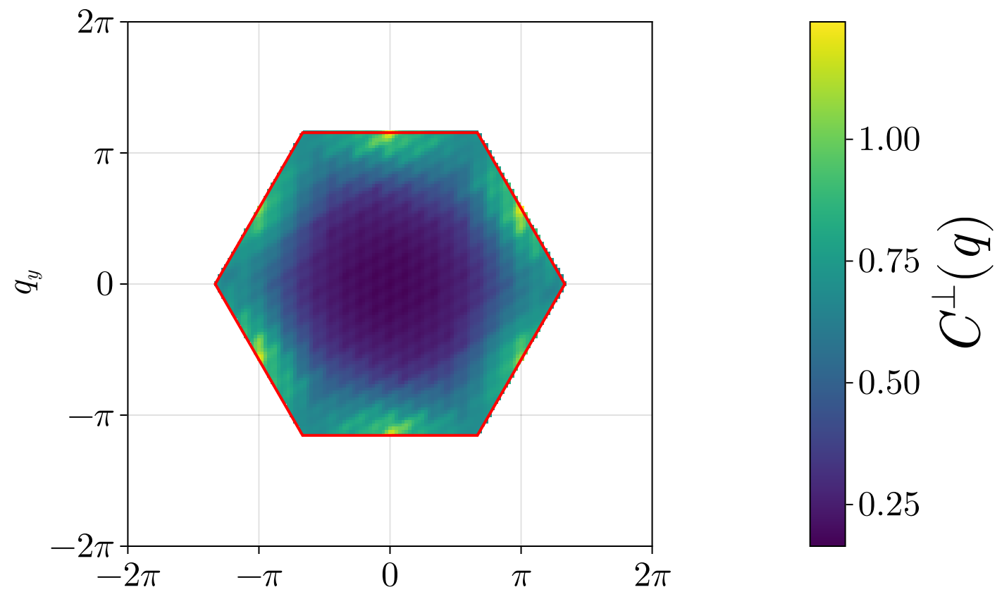
QNG-optimized projected Gutzwiller + D=1 PPEPS: Figure 2(b-i) analogue, J_2/J_1=0.125
