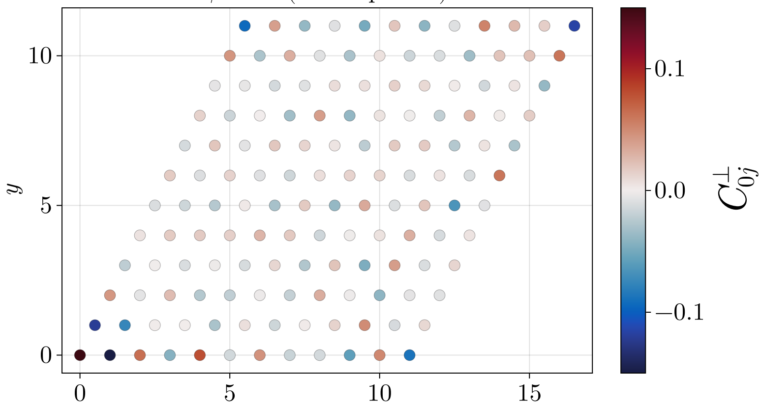
QNG-optimized projected Gutzwiller + D=1 PPEPS: Figure 2(b-i) analogue, J_2/J_1=0.125
