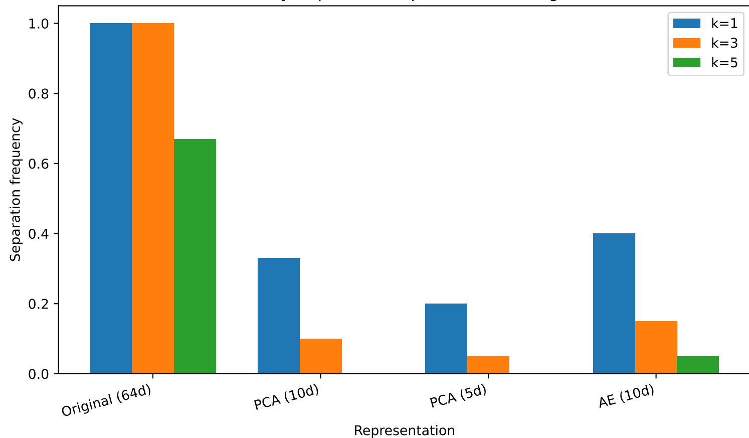
Stability Gap Across Representations (Digits)
