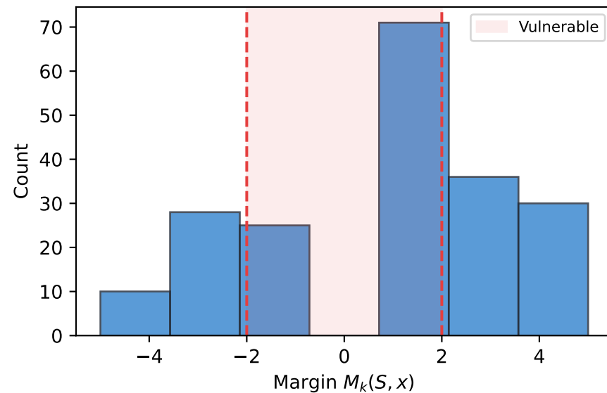
k=5: 96/200 vulnerable (48%)
