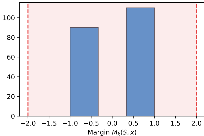
k=1: 200/200 vulnerable (100%)
