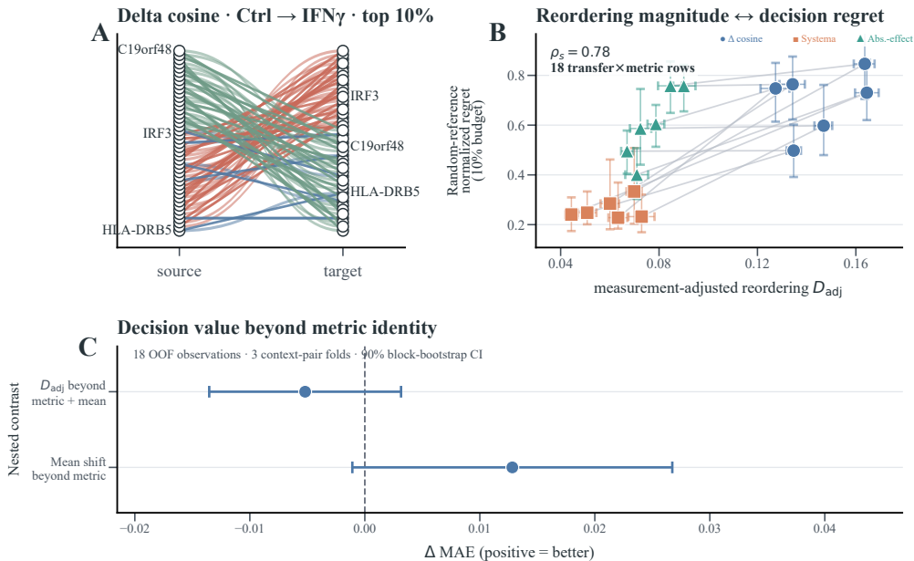
Fig. 4 From reordering to experimental regret
