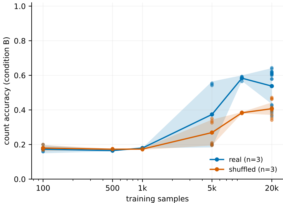
Sample efficiency M1: area-controlled stimuli
