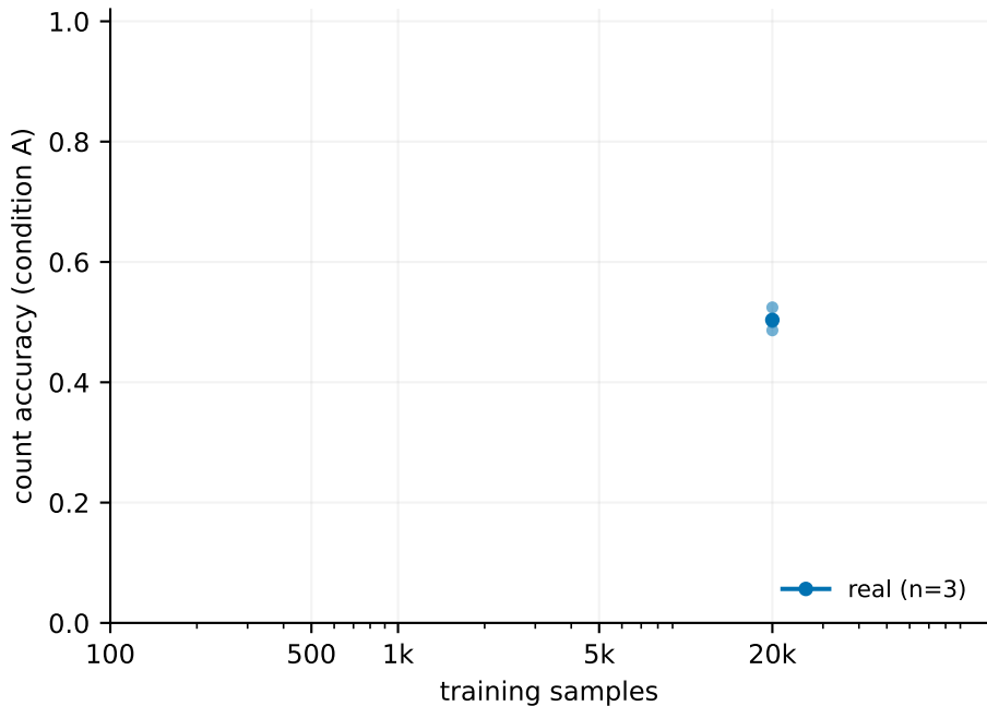
Sample efficiency M0: real vs shuffled (natural stimuli)
