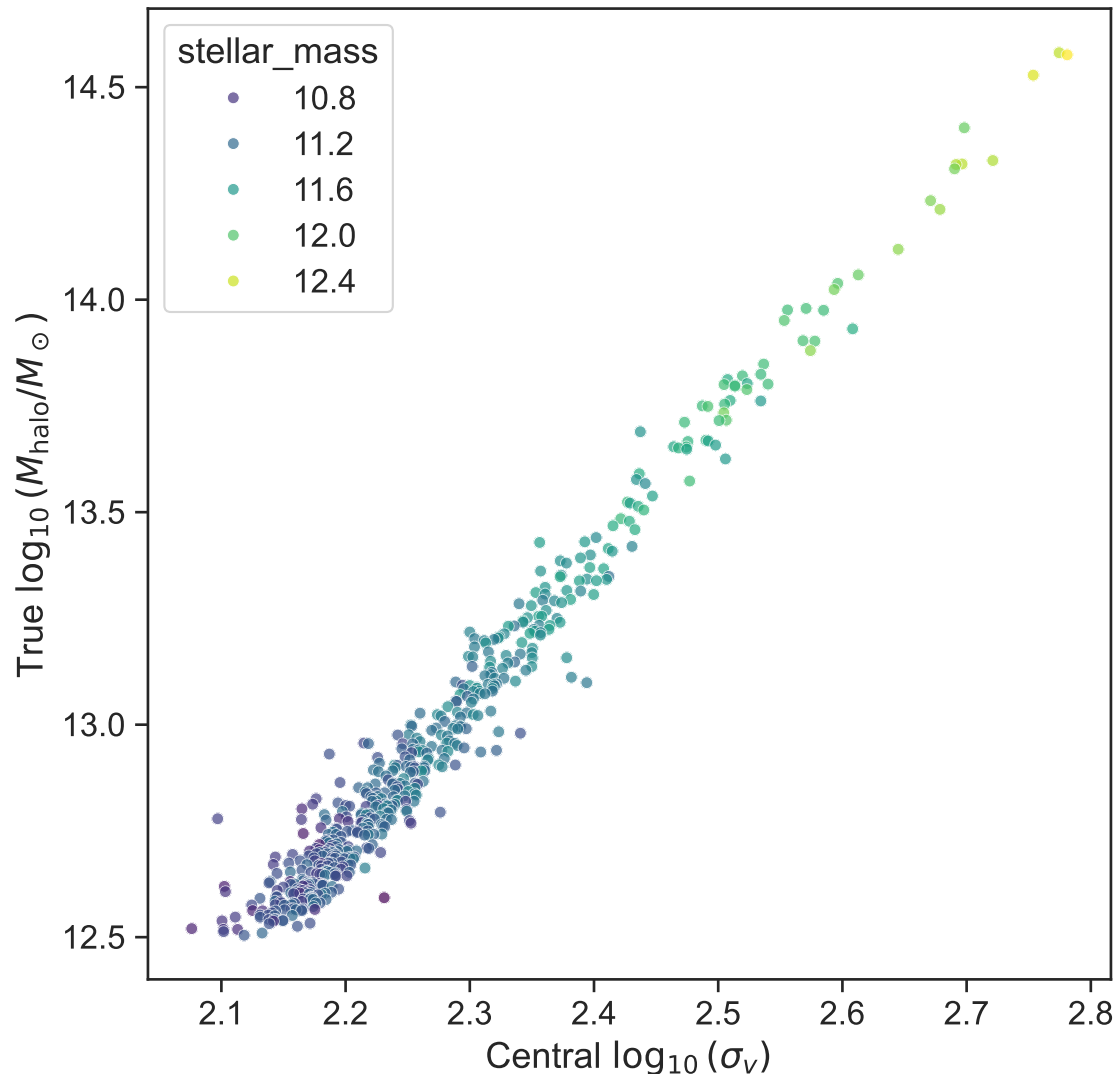
Kinematics vs Halo Mass
