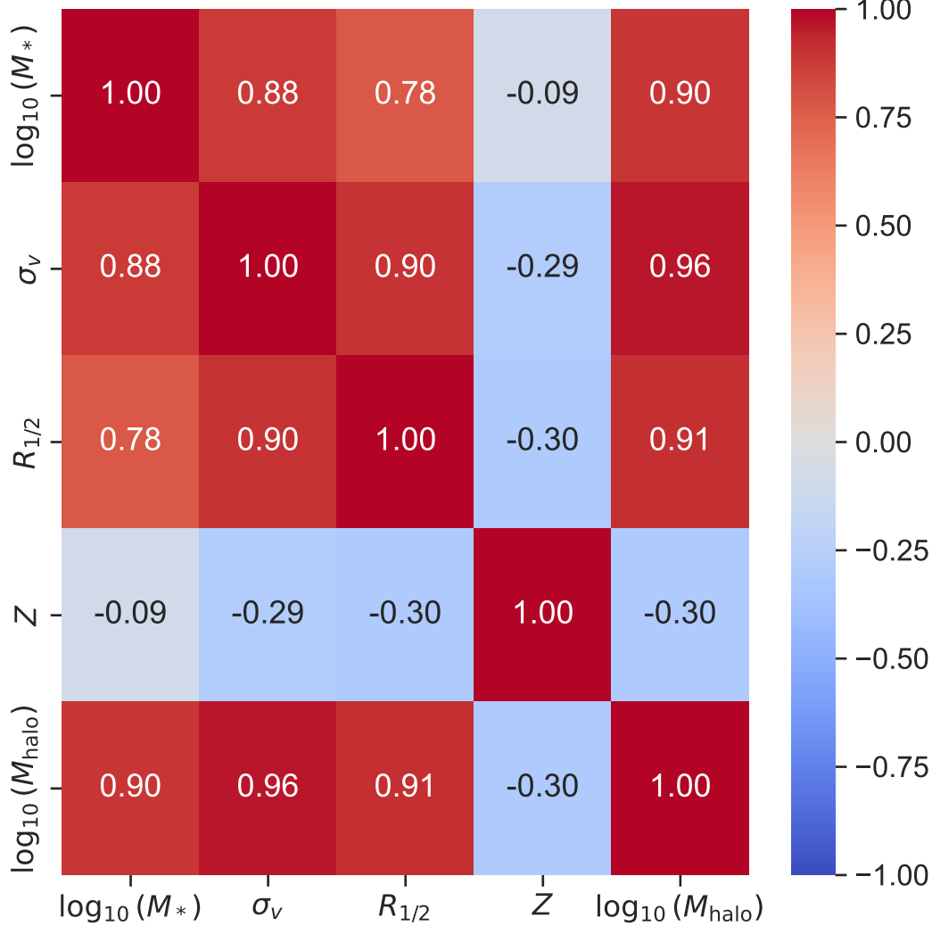
Feature Linear Correlation
