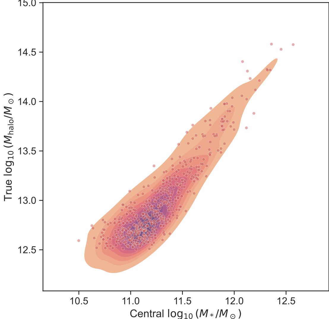
Stellar-to-Halo Mass Relation
