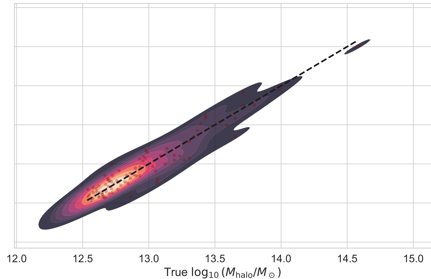
Augmented Best Model R^2 = 0.907 , RMSE = 0.117 dex Scatter \sigma = 0.117 dex
