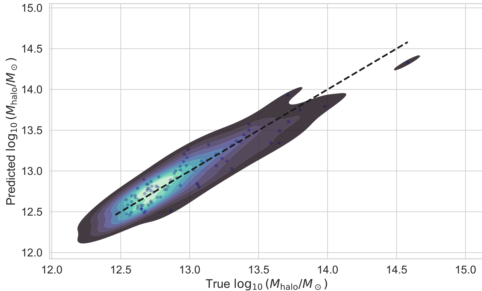
Baseline Best Model R^2 = 0.874 , RMSE = 0.136 dex Scatter \sigma = 0.136 dex
