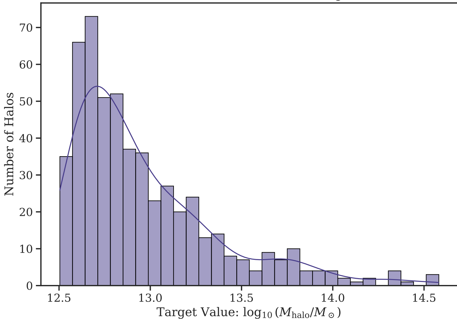
Halo Mass Function (Dataset Targets)
