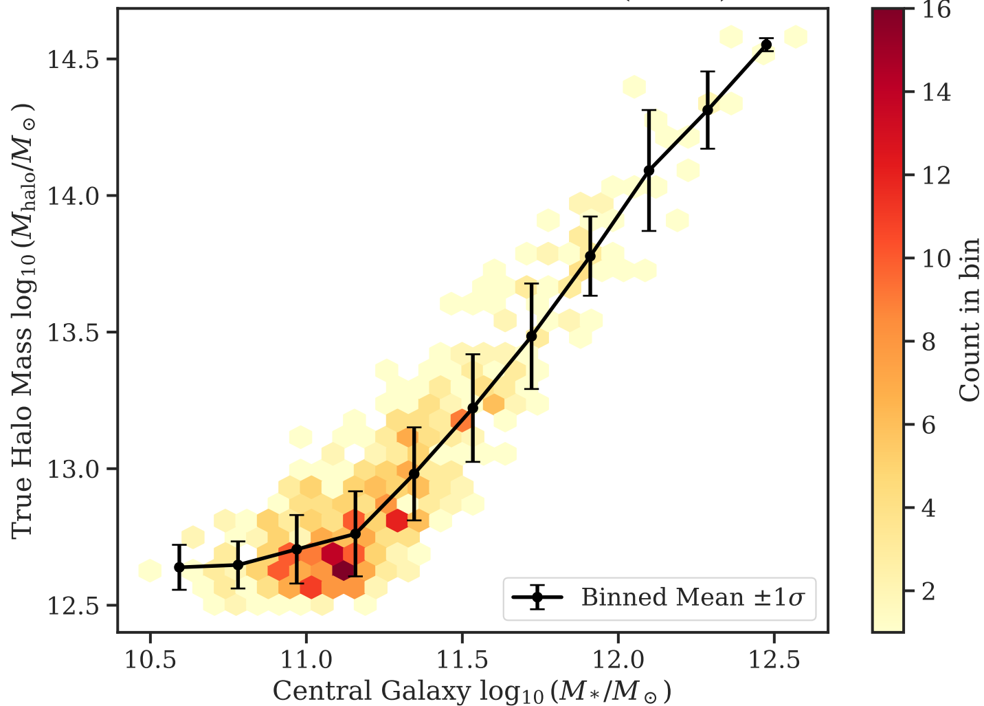
Stellar-to-Halo Mass Relation (SHMR)
