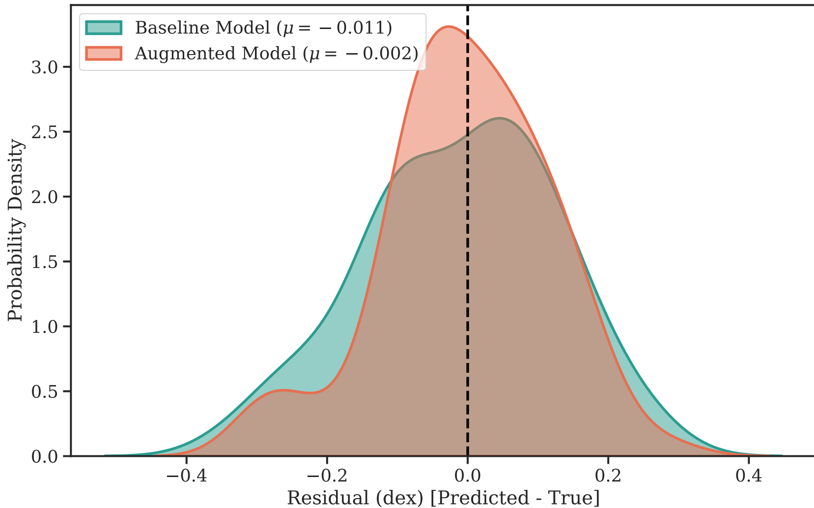
Prediction Residuals Distribution
