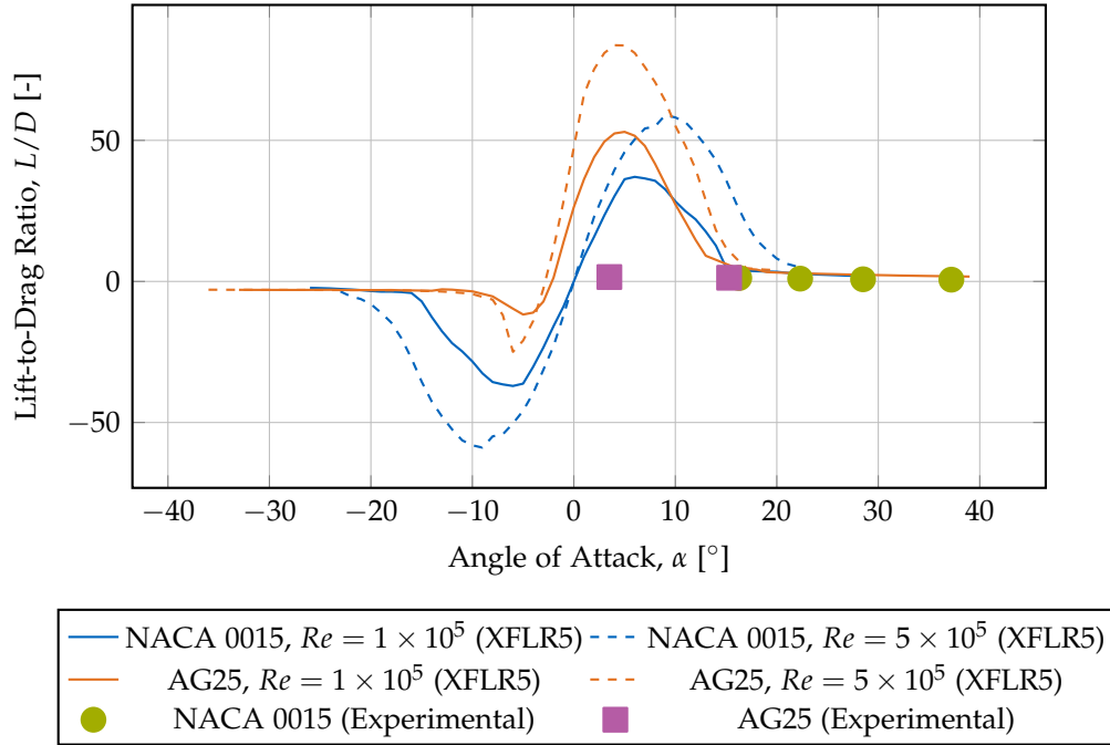
Figure 7.11.: Lift-to-drag ratio comparison highlighting the aerodynamic efficiency of both airfoils. Experimental data shows lower L/D ratios than XFLR5 wing-only predictions due to additional system drag sources (fuselage, propellers, landing gear) not included in the wing simulation. The XFLR5 curves represent wing performance only. NACA 0015 experimental data (green circles) and AG25 experimental data (pink squares) both demonstrate this expected trend. At Re = 1 \times 10^5 , the AG25 wing achieves a remarkable maximum L/D of 53.0 at \alpha \approx 5^\circ , with L/D ratios exceeding 50 between 4^\circ and 6^\circ —substantially higher than the NACA 0015 wing’s maximum L/D of 37.1 at 6^\circ . The experimental measurements at higher angles of attack ( 15^\circ – 40^\circ ) for NACA 0015 and lower angles ( 3^\circ – 15^\circ ) for AG25 reflect their respective operational flight regimes.
