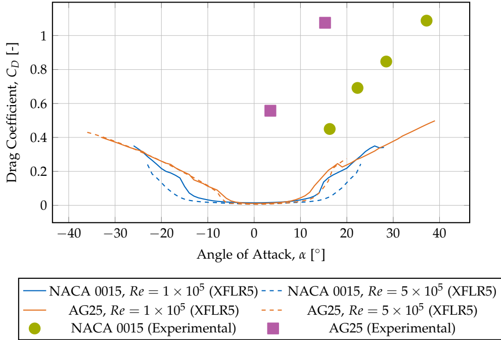
Figure 7.9.: Drag coefficient comparison between NACA 0015 and AG25 airfoils at two Reynolds numbers. Experimental data from flight tests shows higher drag than XFLR5 wing-only simulations, as expected since the experimental values include additional system-level drag sources not present in the simulation: fuselage parasite drag, propeller-induced drag, propeller-wing interference, and landing gear. The XFLR5 predictions represent wing drag only. NACA 0015 experimental data (green circles) and AG25 experimental data (pink squares) both demonstrate this expected trend. At Re = 1 \times 10^5 , the AG25 wing achieves minimum C_D \approx 0.011 near \alpha = -1^\circ , significantly lower than the NACA 0015's C_D \approx 0.015 at \alpha = 0^\circ . The AG25 demonstrates superior low-drag characteristics across the operational angle of attack range.
