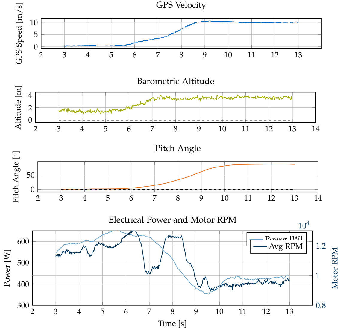
Figure 7.12.: Time-series data from outdoor cruise flight at 10 \text{ ms}^{-1} . From top to bottom: GPS velocity maintains steady cruise speed; barometric altitude variations ( \pm 0.5 \text{ m} ) demonstrate manual altitude control; pitch angle near 87.5^\circ indicates near-level flight; combined plot shows electrical power (blue, left axis) and average motor RPM (teal, right axis) both declining smoothly with airspeed, confirming progressive rotor unloading.
