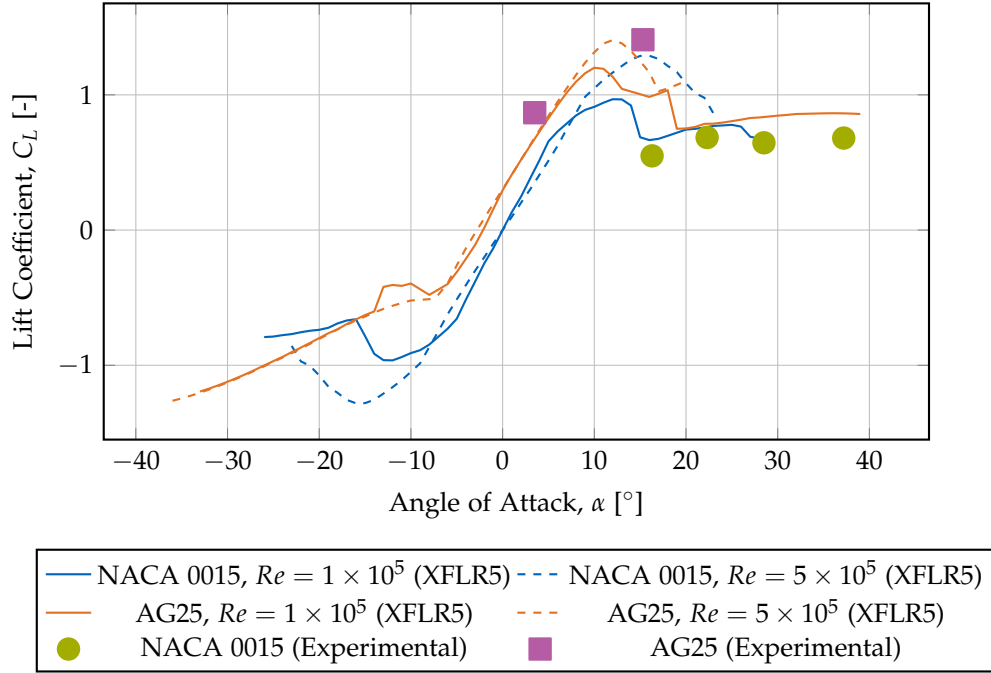
Figure 7.8.: Lift coefficient comparison between NACA 0015 and AG25 airfoils at two Reynolds numbers ( Re = 1 \times 10^5 and Re = 5 \times 10^5 ), computed using XFLR5 with NCrit=5. Experimental data points from flight tests show excellent agreement with XFLR5 predictions for both wing configurations: NACA 0015 (green circles) and AG25 (pink squares), validating the simulation model for lift estimation. At Re = 1 \times 10^5 , the AG25 achieves maximum C_L \approx 1.20 at 10^\circ , while the NACA 0015 reaches C_L \approx 0.97 at 12^\circ .
