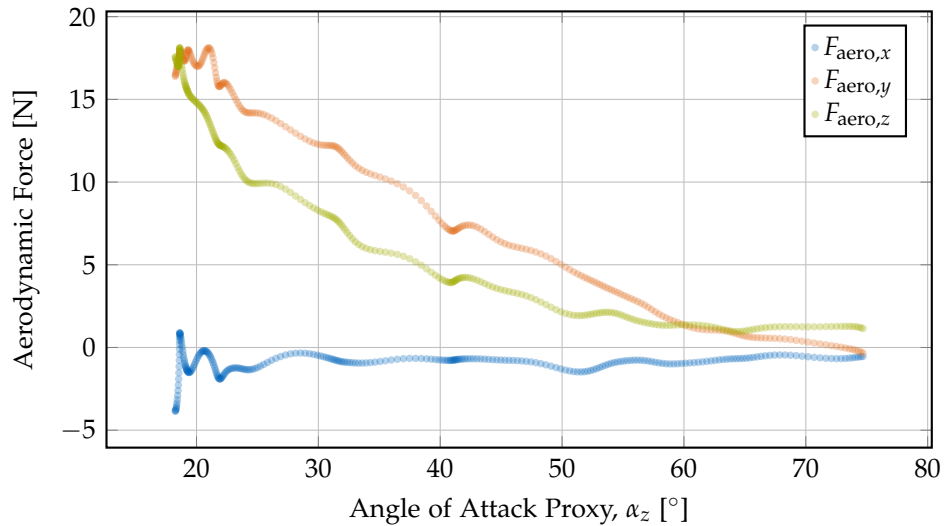
Figure 7.18.: Aerodynamic force components versus kinematic angle-of-attack proxy \alpha_z . The wide angle range reflects transient attitude changes during acceleration.
