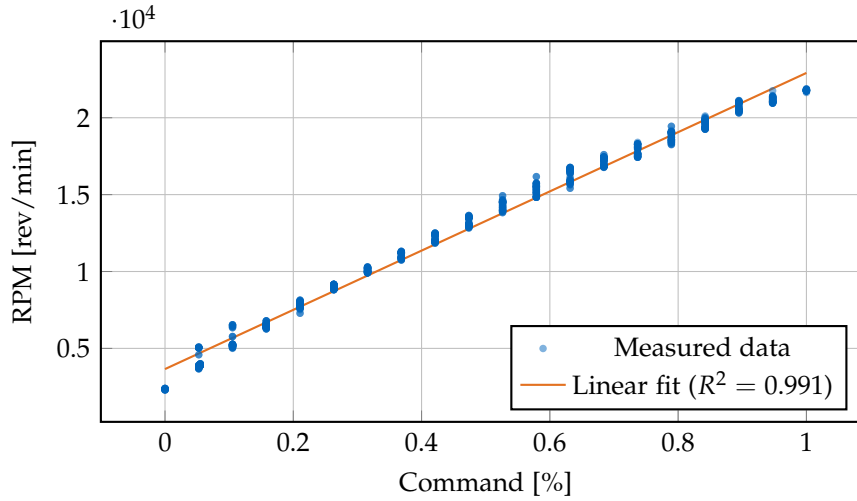
Figure 7.3.: Static mapping between motor command and RPM. The near-linear relationship allows prediction of motor speed from control inputs.
