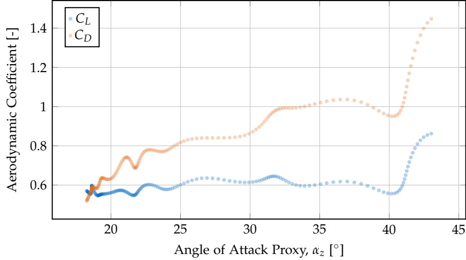
Figure 7.19.: Lift and drag coefficients versus angle-of-attack proxy during straight-line flight (data filtered for V > 5 \text{ m s}^{-1} ). Scatter reflects transient conditions and measurement noise.
