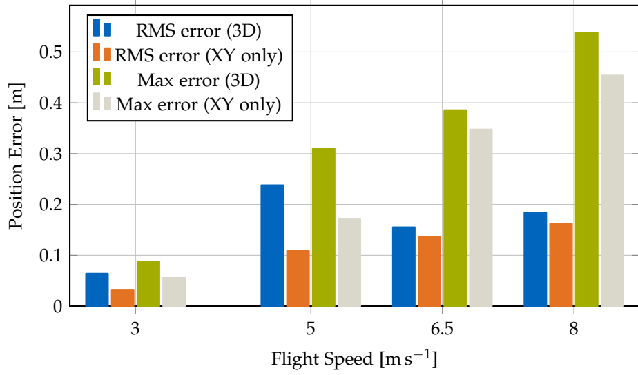
Figure 7.7.: Tracking error as a function of flight speed during circular maneuvers. RMS and maximum errors remain bounded across the speed range; see Table 7.1 for numerical values.
