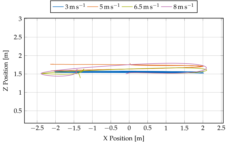
Figure 7.5.: Circular trajectories in XZ plane showing altitude variations during turns at different speeds. The vehicle maintains relatively constant altitude with small vertical deviations.
