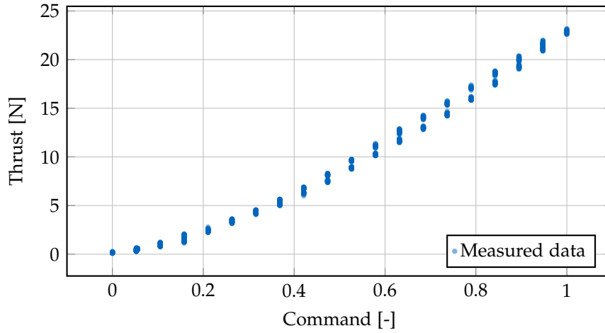
Figure 7.2.: Static thrust as a function of motor command. This relationship is used by the flight controller to map desired thrust into ESC duty cycles.
