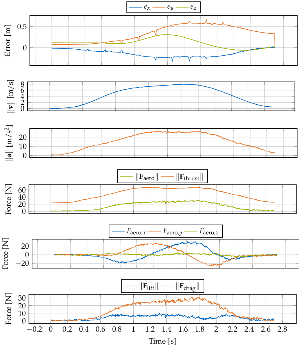
Figure 7.6.: Time-series flight dynamics during one complete circle at 8 \text{ m s}^{-1} . From top: position tracking errors (x, y, z), velocity magnitude, acceleration magnitude, force magnitudes (aerodynamic and thrust), aerodynamic force components in world frame, and lift and drag force magnitudes. The bounded errors and smooth force profiles demonstrate stable control despite time-varying aerodynamic loads approaching 6 N.
