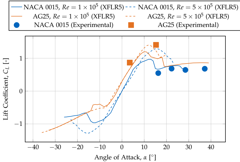
Figure 7.9.: Lift coefficient C_L versus angle of attack for NACA 0015 and AG25 at two Reynolds numbers, comparing XFLR5 predictions with coefficients extracted from flight tests. Experimental lift closely follows the XFLR5 curves for both airfoils.
