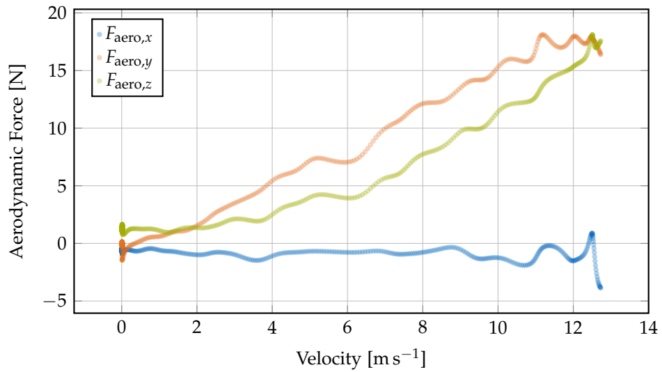
Figure 7.17.: Aerodynamic force components in world frame versus flight speed during straight-line acceleration. The scatter reflects transient flight conditions across the full speed envelope.
