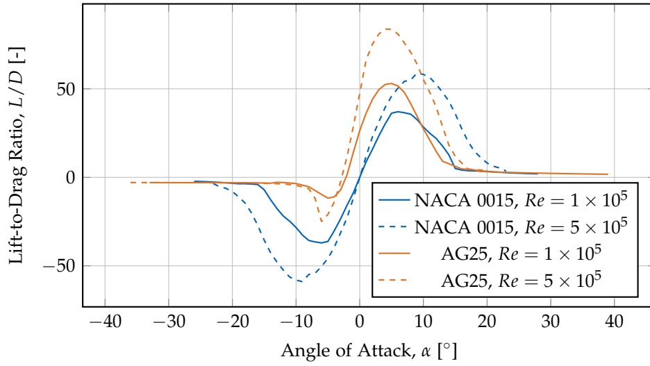
Figure 7.14: Lift-to-drag ratio comparison highlighting the aerodynamic efficiency of both airfoils. At Re = 1 \times 10^5 , the AG25 achieves a remarkable maximum L/D of 53.0 at \alpha \approx 5^\circ , with L/D ratios exceeding 50 between 4^\circ and 6^\circ —substantially higher than the NACA 0015’s maximum L/D of 37.1 at 6^\circ . At typical cruise angles ( 4^\circ – 6^\circ ), the AG25 maintains L/D ratios above 50, representing a 30–43% improvement over the NACA 0015 baseline and enabling significantly more efficient forward flight.
