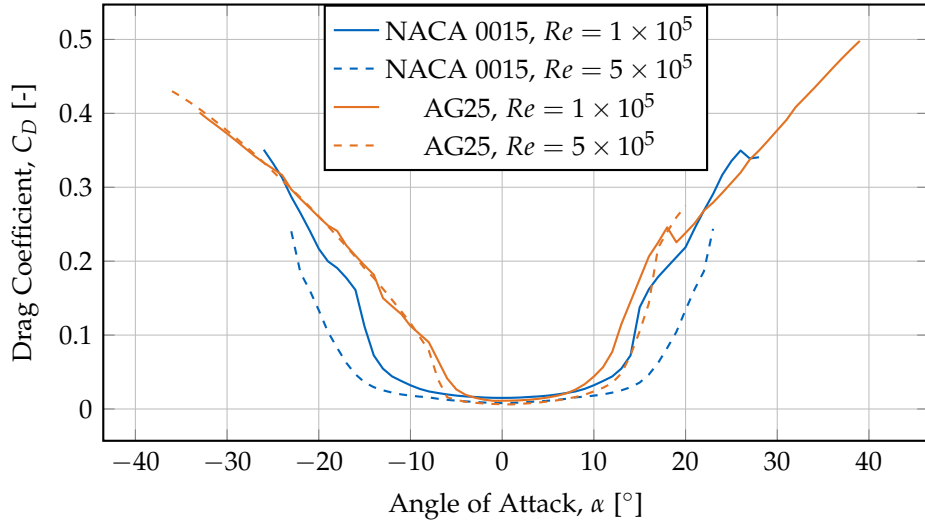
Figure 7.12: Drag coefficient comparison between NACA 0015 and AG25 airfoils at two Reynolds numbers. At Re = 1 \times 10^5 , the AG25 achieves minimum C_D \approx 0.011 near \alpha = -1^\circ , significantly lower than the NACA 0015's C_D \approx 0.015 at \alpha = 0^\circ . The AG25 demonstrates superior low-drag characteristics across the operational angle of attack range, with drag coefficients approximately 25-30% lower than the NACA 0015 baseline.
