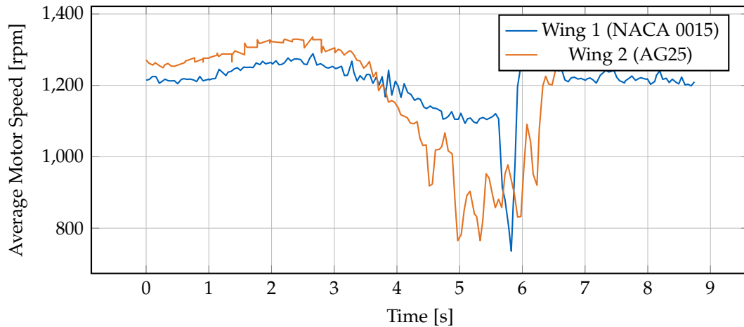
Figure 7.15: Per-motor rotation speeds during hover and straight-line cruise. Key values (per motor): Wing 1 — hover 1200 rpm, cruise ( 9 \text{ m/s} ) 1150 rpm; Wing 2 — hover 1260 rpm, cruise ( 9 \text{ m/s} ) 1000 rpm. The cruise unloading of Wing 2's rotors indicates a larger aerodynamic contribution to lift at forward speed.
