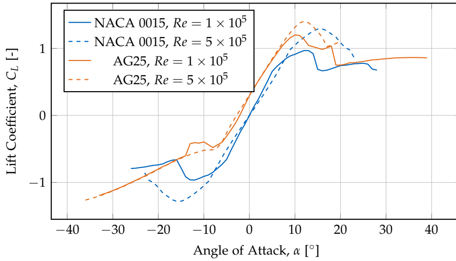
Figure 7.11: Lift coefficient comparison between NACA 0015 and AG25 airfoils at two Reynolds numbers ( Re = 1 \times 10^5 and Re = 5 \times 10^5 ), computed using XFLR5 with NCrit=5. At Re = 1 \times 10^5 , the AG25 achieves maximum C_L \approx 1.20 at 10^\circ , while the NACA 0015 reaches C_L \approx 0.97 at 12^\circ . Both airfoils show improved performance at higher Reynolds numbers, with more gradual stall characteristics and higher maximum lift coefficients.
