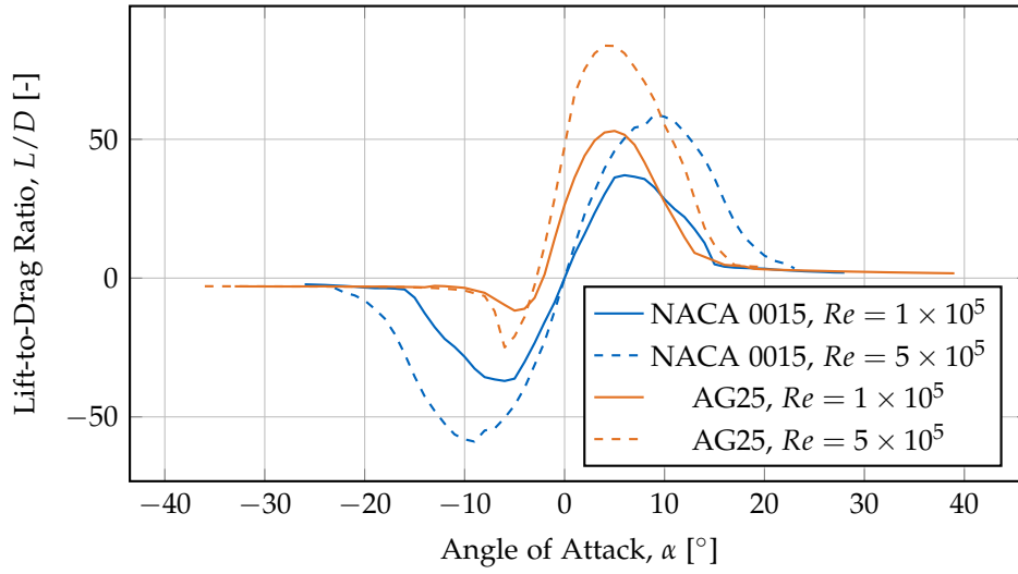
Figure 7.10: Lift-to-drag ratio comparison highlighting the aerodynamic efficiency of both airfoils. At Re = 1 \times 10^5 , the AG25 achieves a remarkable maximum L/D of 53.0 at \alpha \approx 5^\circ , with L/D ratios exceeding 50 between 4^\circ and 6^\circ —substantially higher than the NACA 0015’s maximum L/D of 37.1 at 6^\circ . At typical cruise angles ( 4^\circ – 6^\circ ), the AG25 maintains L/D ratios above 50, representing a 30–43% improvement over the NACA 0015 baseline and enabling significantly more efficient forward flight.
