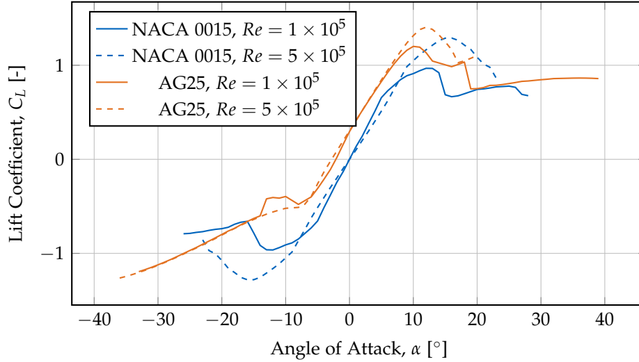
Figure 7.7: Lift coefficient comparison between NACA 0015 and AG25 airfoils at two Reynolds numbers ( Re = 1 \times 10^5 and Re = 5 \times 10^5 ), computed using XFLR5 with NCrit=5. At Re = 1 \times 10^5 , the AG25 achieves maximum C_L \approx 1.20 at 10^\circ , while the NACA 0015 reaches C_L \approx 0.97 at 12^\circ . Both airfoils show improved performance at higher Reynolds numbers, with more gradual stall characteristics and higher maximum lift coefficients.
