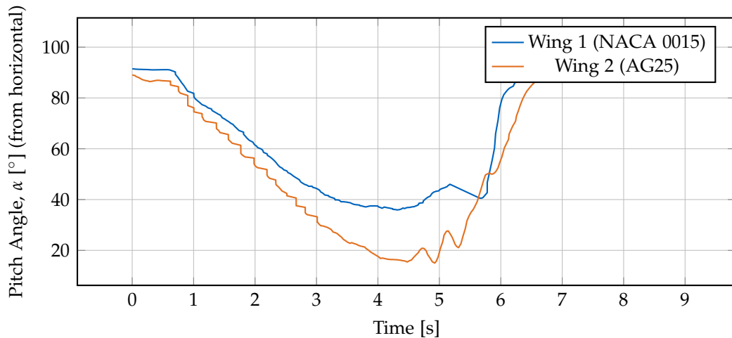
Figure 7.13.: Pitch-angle time histories (angles measured from the horizontal plane). The AG25-equipped vehicle (Wing 2) reaches a minimum pitch angle of approximately 15^\circ , while the NACA 0015 baseline (Wing 1) reaches a minimum of approximately 36^\circ . These extrema indicate that Wing 2 can sustain lift at much lower nose-up attitudes.
