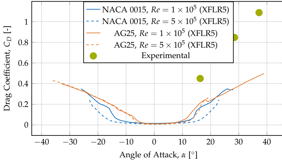
Figure 7.9.: Drag coefficient comparison between NACA 0015 and AG25 airfoils at two Reynolds numbers. Experimental data from flight tests (green markers) shows higher drag than XFLR5 wing-only simulations, as expected since the experimental values include additional system-level drag sources not present in the simulation: fuselage parasite drag, propeller-induced drag, propeller-wing interference, and landing gear. The XFLR5 predictions represent wing drag only. At Re = 1 \times 10^5 , the AG25 wing achieves minimum C_D \approx 0.011 near \alpha = -1^\circ , significantly lower than the NACA 0015's C_D \approx 0.015 at \alpha = 0^\circ . The AG25 demonstrates superior low-drag characteristics across the operational angle of attack range.
