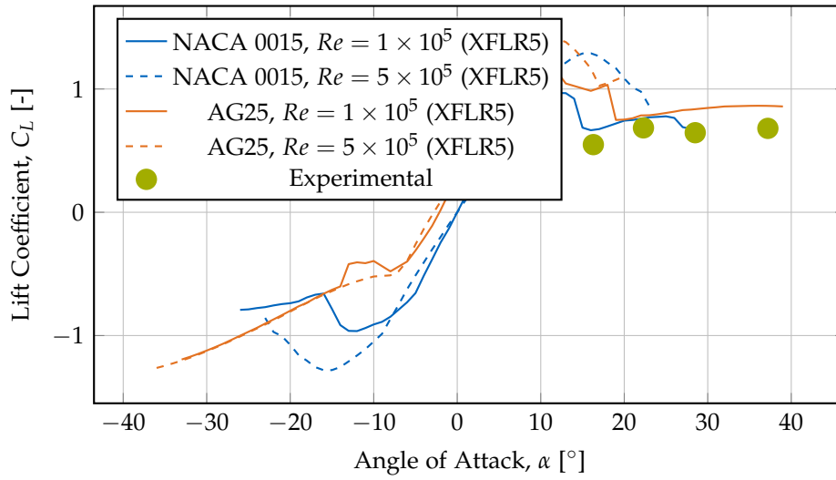
Figure 7.8.: Lift coefficient comparison between NACA 0015 and AG25 airfoils at two Reynolds numbers ( Re = 1 \times 10^5 and Re = 5 \times 10^5 ), computed using XFLR5 with NCrit=5. Experimental data points from flight tests (green markers) show excellent agreement with XFLR5 predictions, validating the simulation model for lift estimation. At Re = 1 \times 10^5 , the AG25 achieves maximum C_L \approx 1.20 at 10^\circ , while the NACA 0015 reaches C_L \approx 0.97 at 12^\circ .
