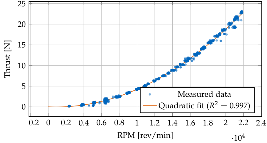
Figure 7.1.: Thrust vs RPM with zero-offset corrected quadratic fit. An offset of -0.996\text{ N} was applied to ensure zero thrust at zero RPM.
