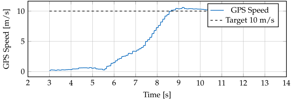
Figure 7.14.: GPS velocity during outdoor cruise flight. The platform maintains steady 10\text{ m s}^{-1} forward speed with minimal oscillation under manual control, demonstrating the pilot's ability to achieve consistent cruise conditions for efficiency testing.
