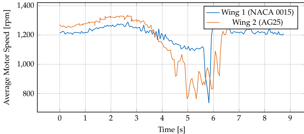
Figure 7.12.: Per-motor rotation speeds during hover and straight-line cruise. Key values (per motor): Wing 1 — hover 1200 rpm, cruise (9 m/s) 1150 rpm; Wing 2 — hover 1260 rpm, cruise (9 m/s) 1000 rpm. The cruise unloading of Wing 2's rotors indicates a larger aerodynamic contribution to lift at forward speed.
