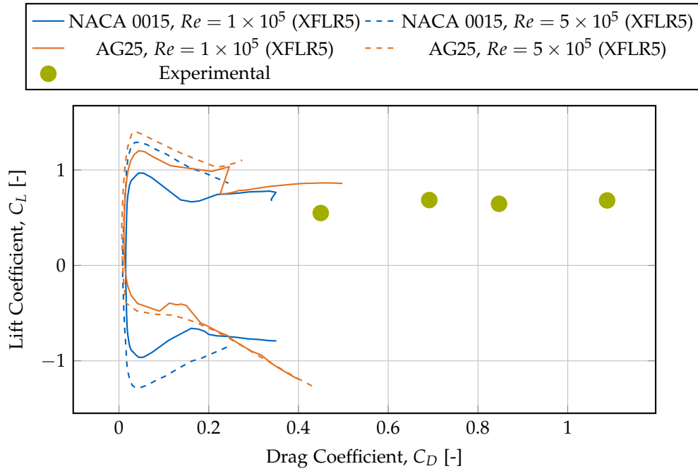
Figure 7.14.: Drag polar comparison showing the relationship between lift and drag coefficients. Curves shifted toward the left and top indicate better aerodynamic efficiency (higher lift for given drag). Experimental data (green markers) shows lower lift coefficients and higher drag coefficients than XFLR5 predictions, reflecting system-level effects including fuselage drag, propeller-wing interference, and three-dimensional flow effects not captured in 2D airfoil analysis. At both Reynolds numbers, the AG25 demonstrates dramatically superior efficiency with the drag polar shifted significantly leftward compared to NACA 0015, achieving higher lift coefficients at substantially lower drag penalties.
