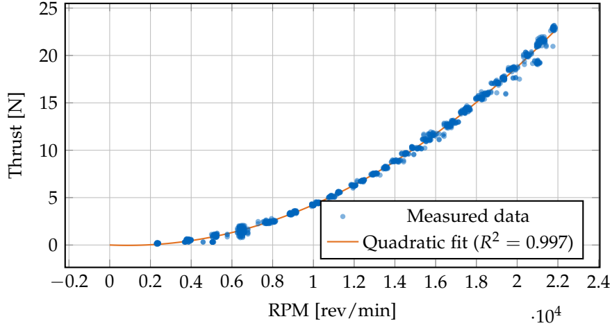
Figure 7.1.: Thrust vs RPM with zero-offset corrected quadratic fit. An offset of -0.996 N was applied to ensure zero thrust at zero RPM.
