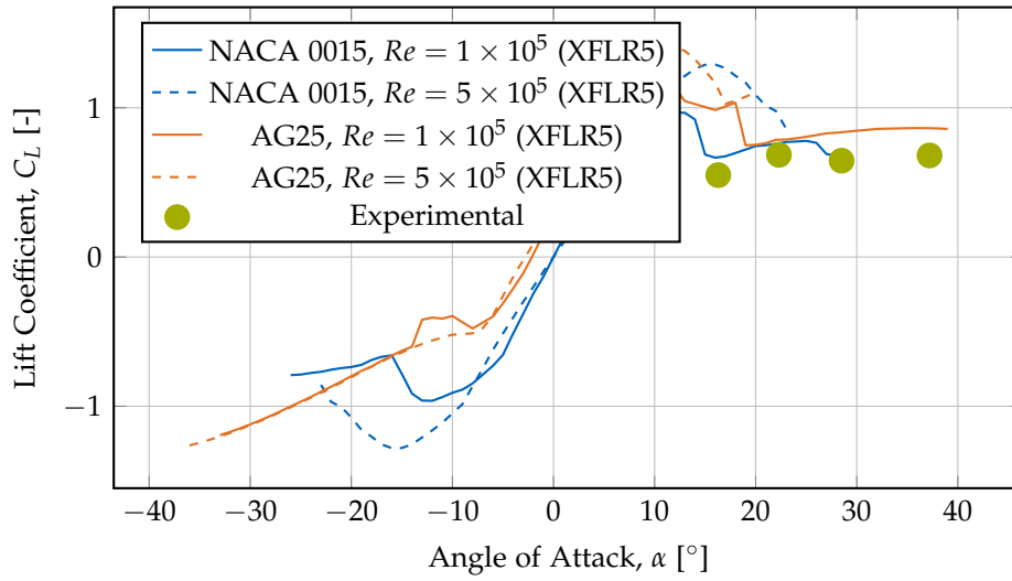
Figure 7.12.: Lift coefficient comparison between NACA 0015 and AG25 airfoils at two Reynolds numbers ( Re = 1 \times 10^5 and Re = 5 \times 10^5 ), computed using XFLR5 with NCrit=5 . Experimental data points from flight tests (green markers) show lower lift coefficients than XFLR5 predictions, likely due to propeller-wing interference effects, fuselage blockage, and the relatively low aspect ratio of the X-configuration. At Re = 1 \times 10^5 , the AG25 achieves maximum C_L \approx 1.20 at 10^\circ , while the NACA 0015 reaches C_L \approx 0.97 at 12^\circ .
