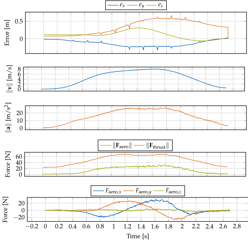
Figure 7.6.: Time-series flight dynamics during one complete circle at 8 \text{ m s}^{-1} . From top: position tracking errors ( x , y , z ), velocity magnitude, acceleration magnitude, force magnitudes (aerodynamic and thrust), and aerodynamic force components in world frame. The bounded errors and smooth force profiles demonstrate stable control despite time-varying aerodynamic loads approaching 6 \text{ N} .
