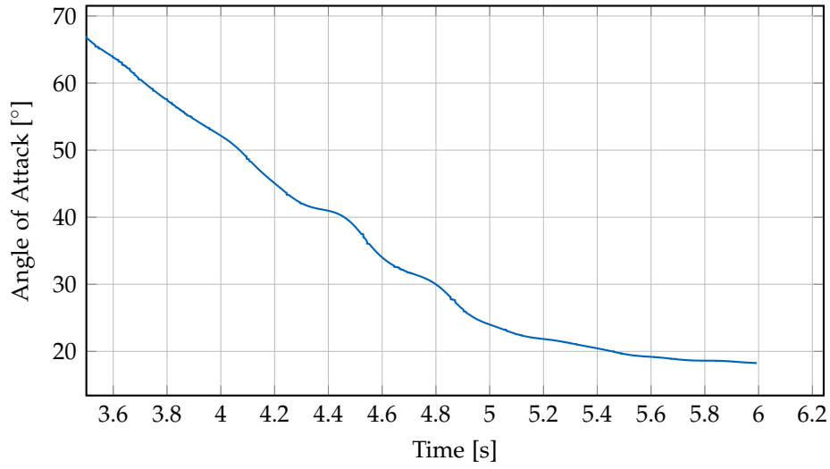
Figure 7.16.: Kinematic angle-of-attack proxy \alpha_z (angle between body z-axis and velocity vector) versus time. Data begins at 3.5 s as the angle of attack is undefined during hover due to negligible velocity.
