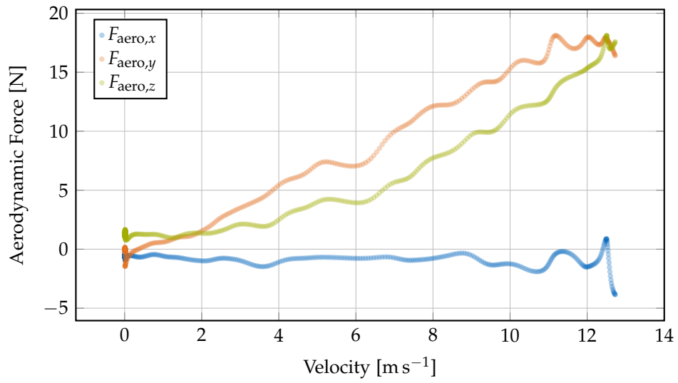
Figure 7.17.: Aerodynamic force components in world frame versus flight speed during straight-line acceleration. The scatter reflects transient flight conditions across the full speed envelope.
