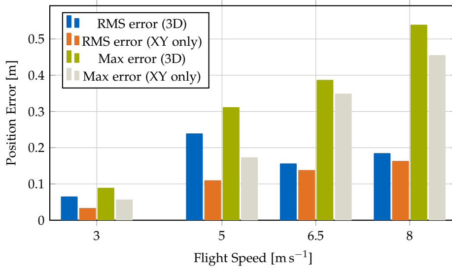
Figure 7.7.: Tracking error as a function of flight speed during circular maneuvers. RMS and maximum errors remain bounded across the speed range; see Table 7.1 for numerical values.
