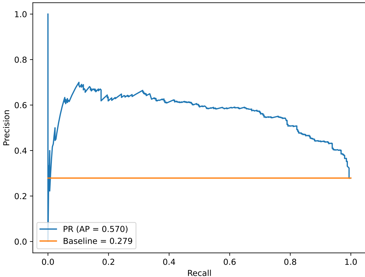
Precision-Recall Curve (2024 Holdout)
