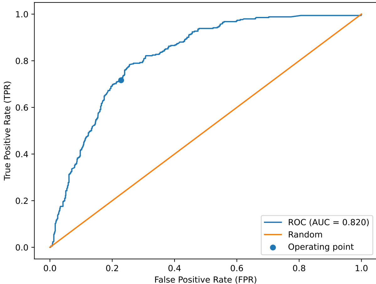
ROC Curve (2024 Holdout)
