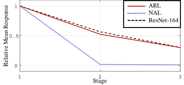
Figure 4: The mean absolute response of output features in each stage.
