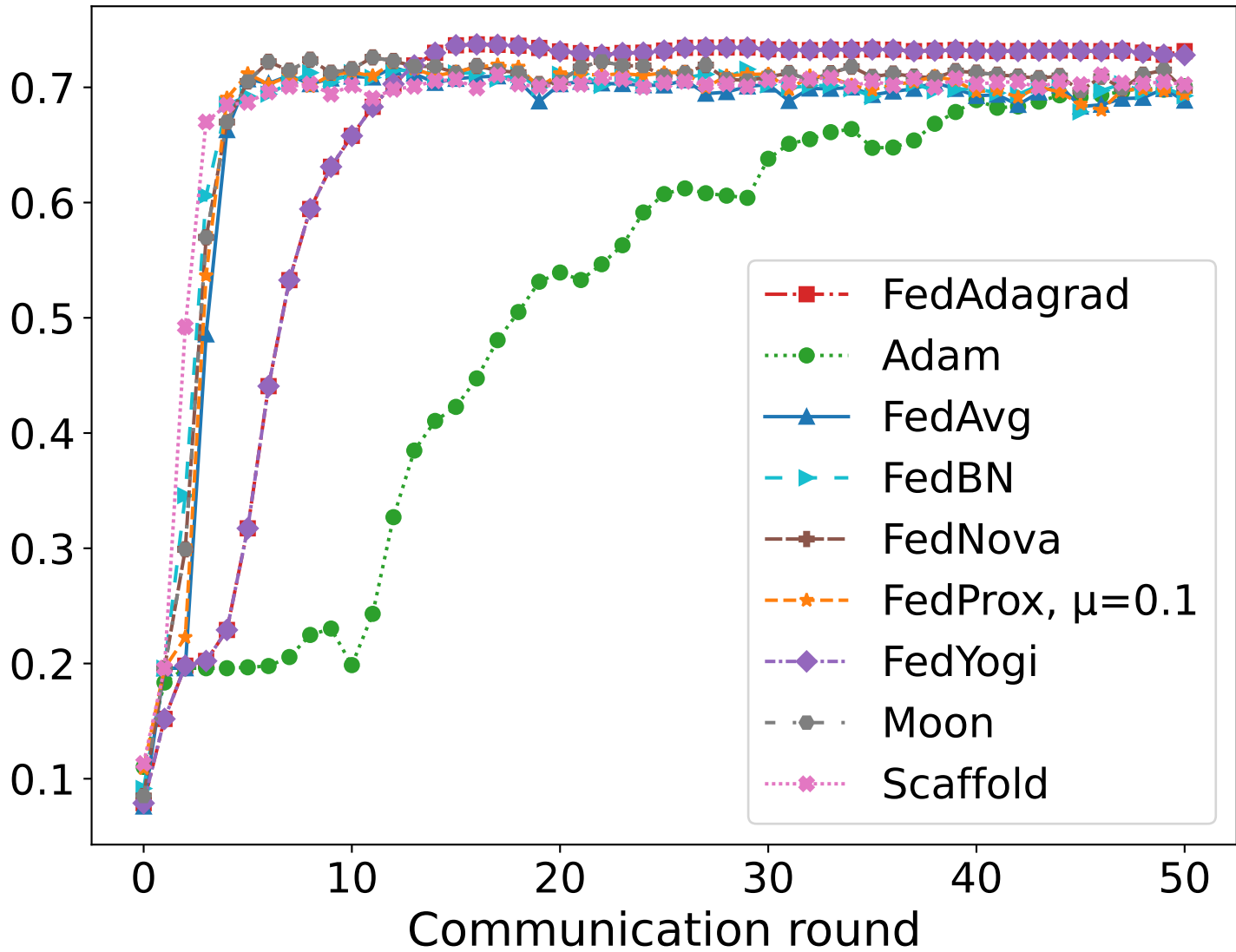
Test accuracy
