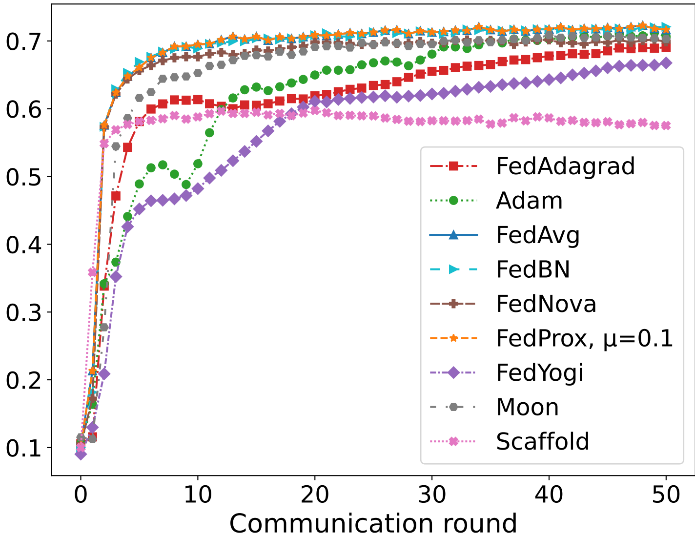
Test accuracy
