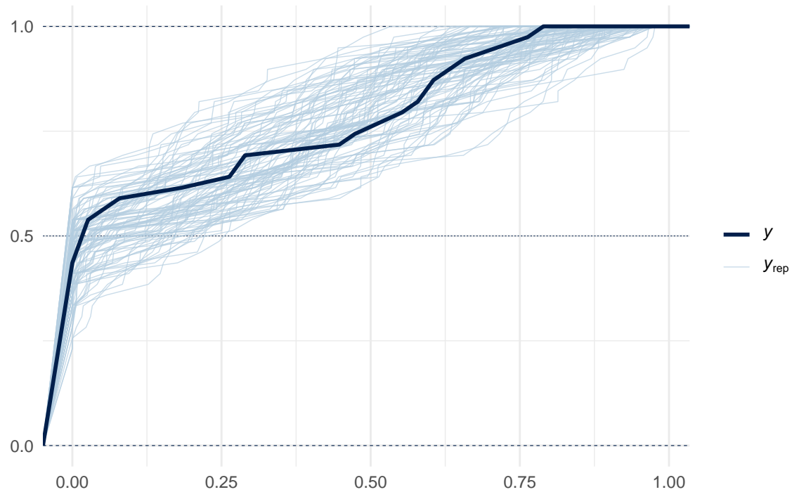
PPC ECDF: zero_inflated_beta
