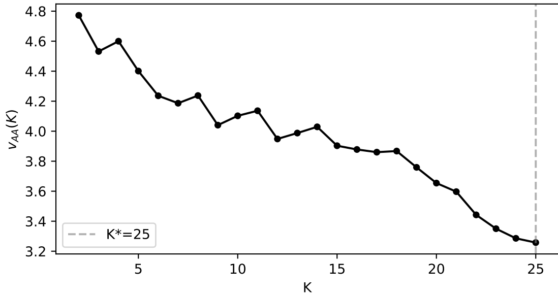
Suleman (2017) criterion
