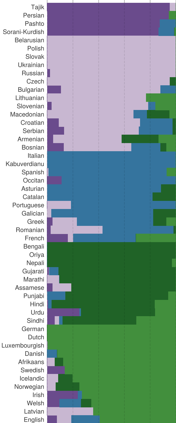
Acoustic archetypes
