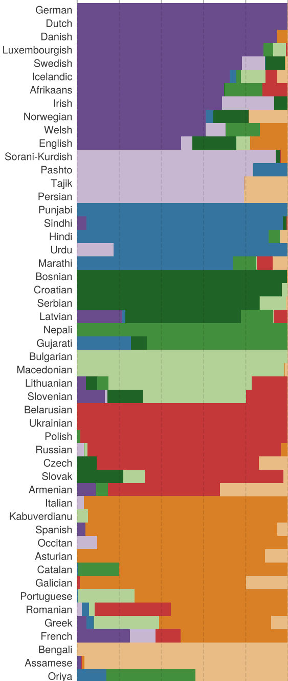
Acoustic archetypes
