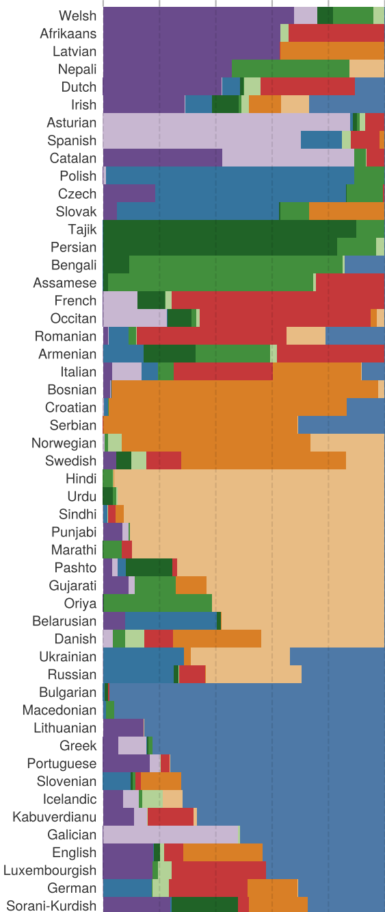
NMF components
